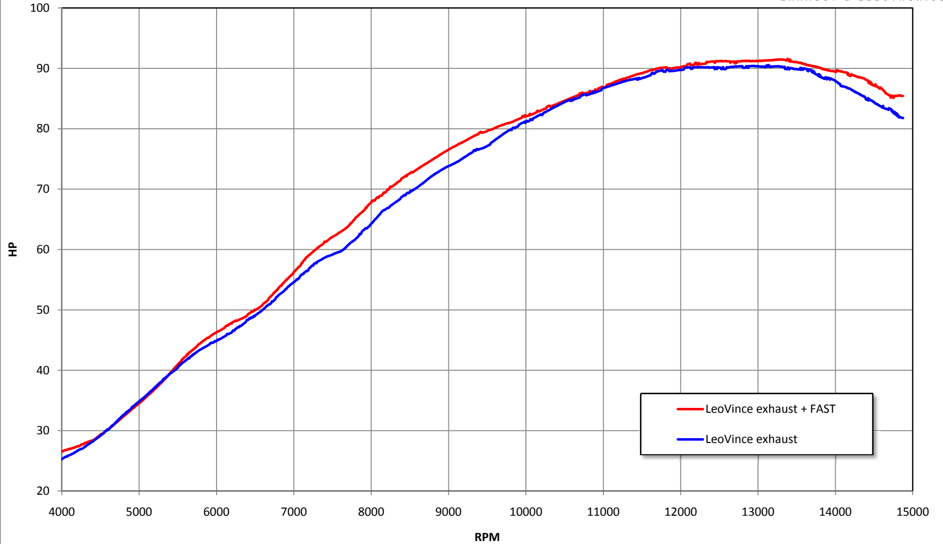
Honda CBR 600 RR i.e. (2009-2010) - "Corsa" full-system with dB killer - 50% Throttle test
