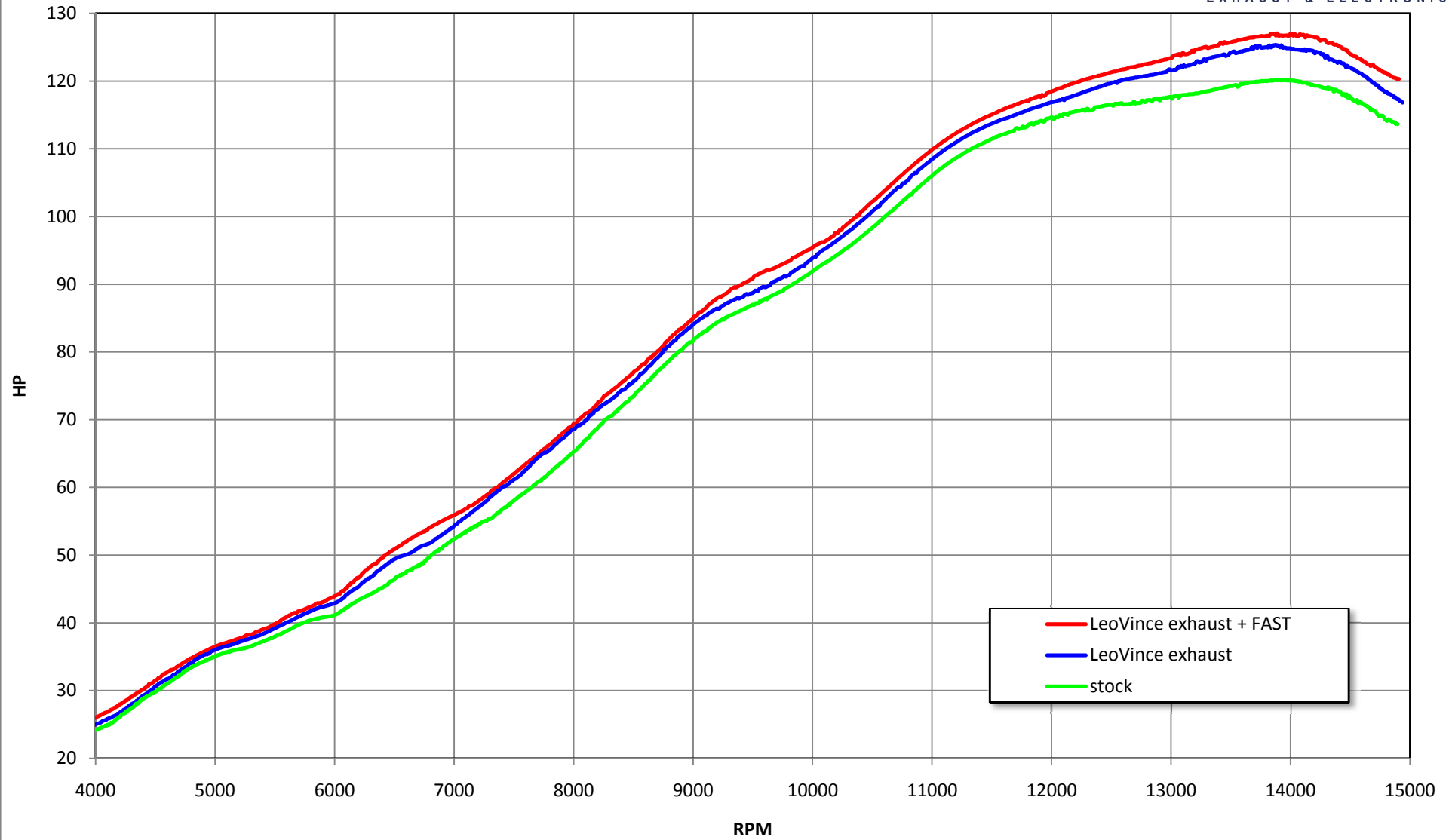
Honda CBR 600 RR i.e. (2009-2010) - FACTORY, OVAL slip-on without dB killer - Full Throttle test
