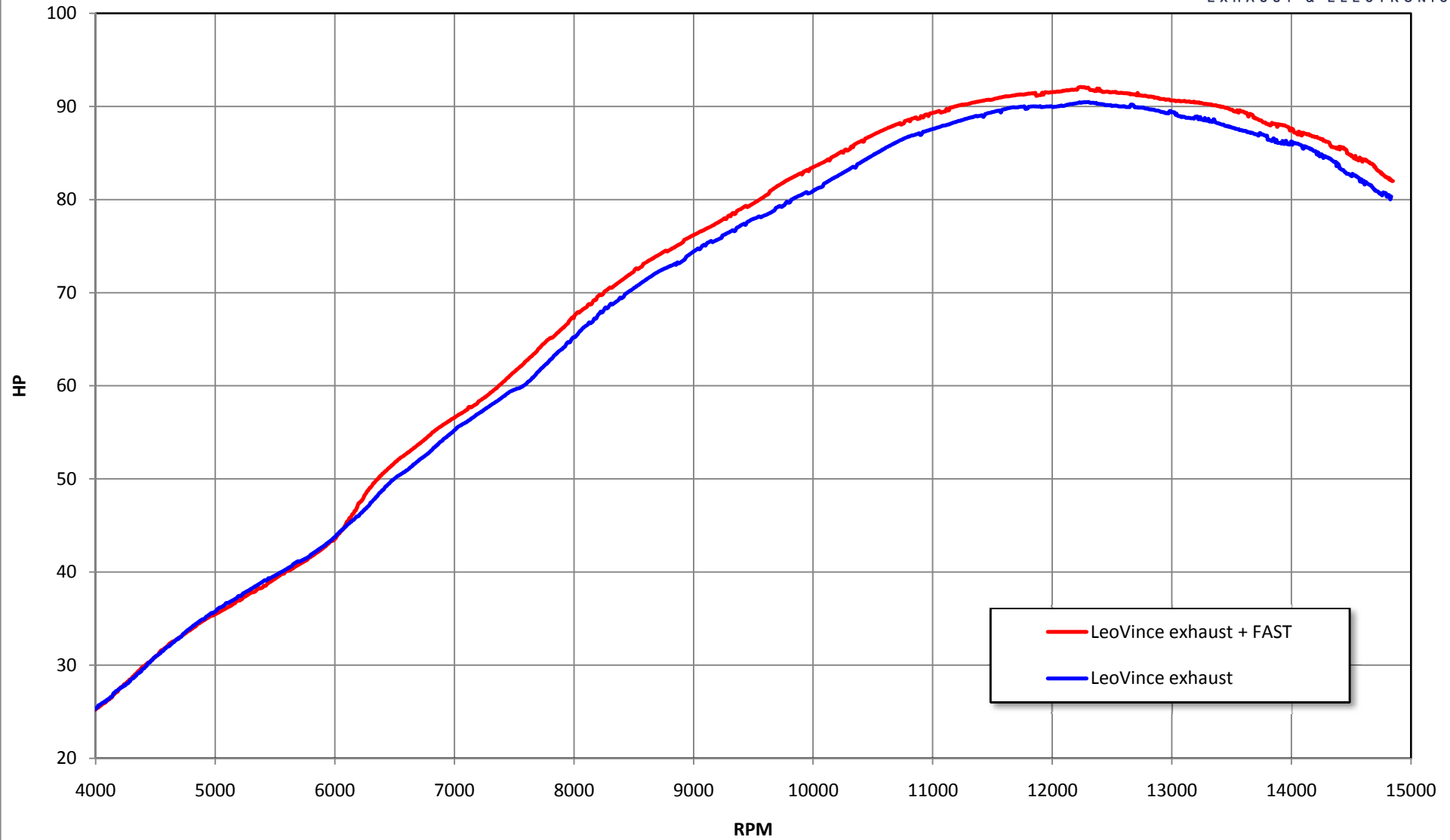
Honda CBR 600 RR i.e. (2009-2010) - FACTORY, OVAL slip-on without dB killer - 50% Throttle test
